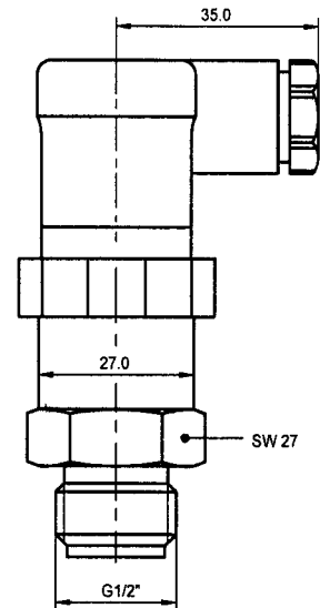
P 10 / P 21 G1/2" 1.4404
